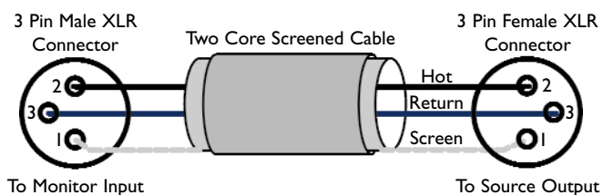
Diagram 2 - balanced cable
