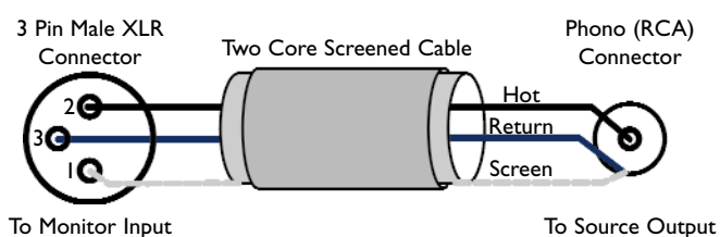
Diagram 3 - unbalanced cable
