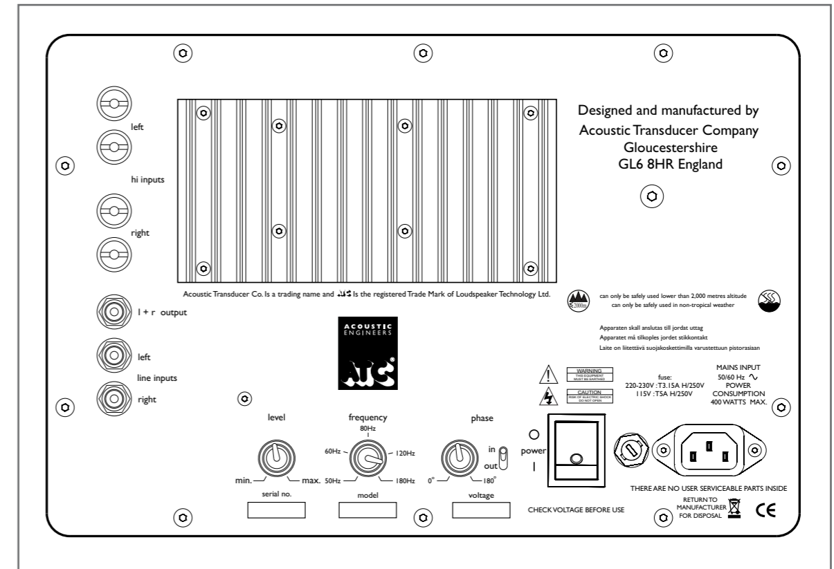
Fig. 2 C1 Sub Amplifier Rear Panel
