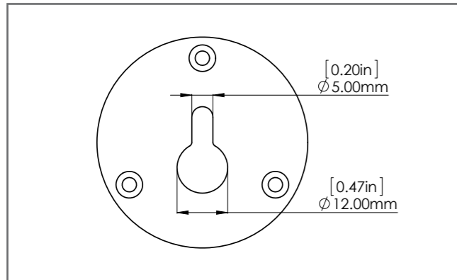
Fig. 3 “Keyhole” fixing for wall mounting
